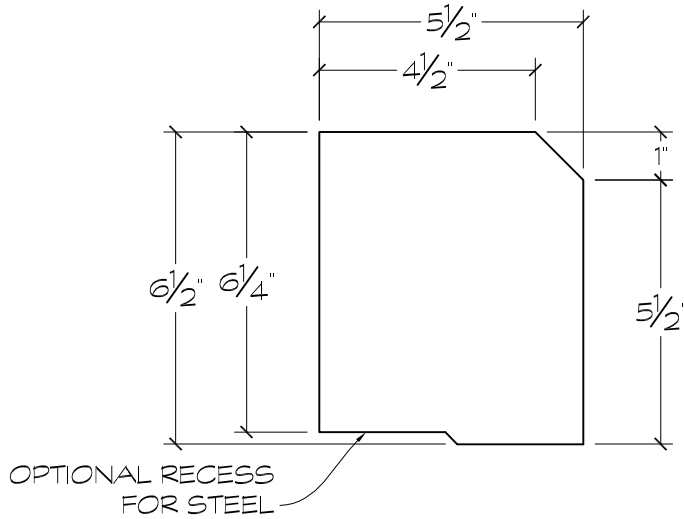
CROSS SECTION
