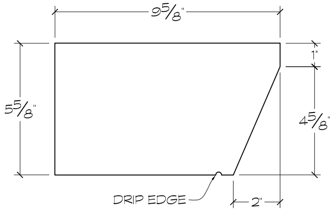
CROSS SECTION
