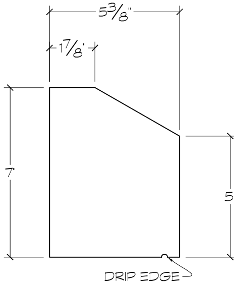
CROSS SECTION
