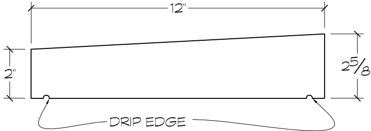
CROSS SECTION
