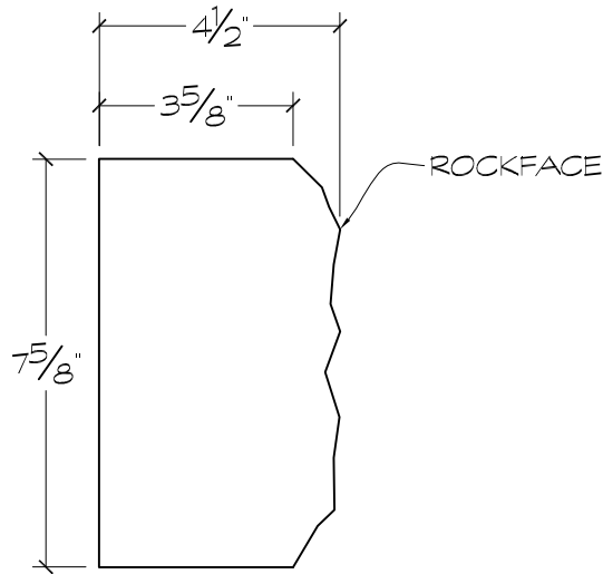
CROSS SECTION
