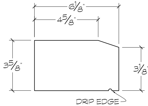
CROSS SECTION
